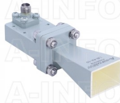
LB-42-10-C-SF Standard Gain Horn Antenna 18-26.5GHz 10dB Gain SMA Female
