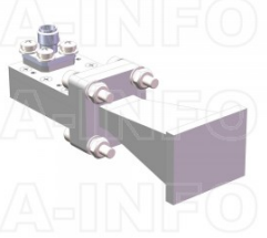
LB-42-10-C-KFSPO Standard Gain Horn Antenna 18-26.5GHz 10dB Gain 2.92mm Female
